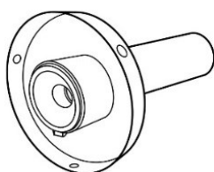
SOUND REDUCER (1)
