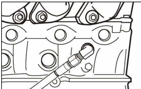
Connect the hose to the fitting on the cylinder block installed earlier.
